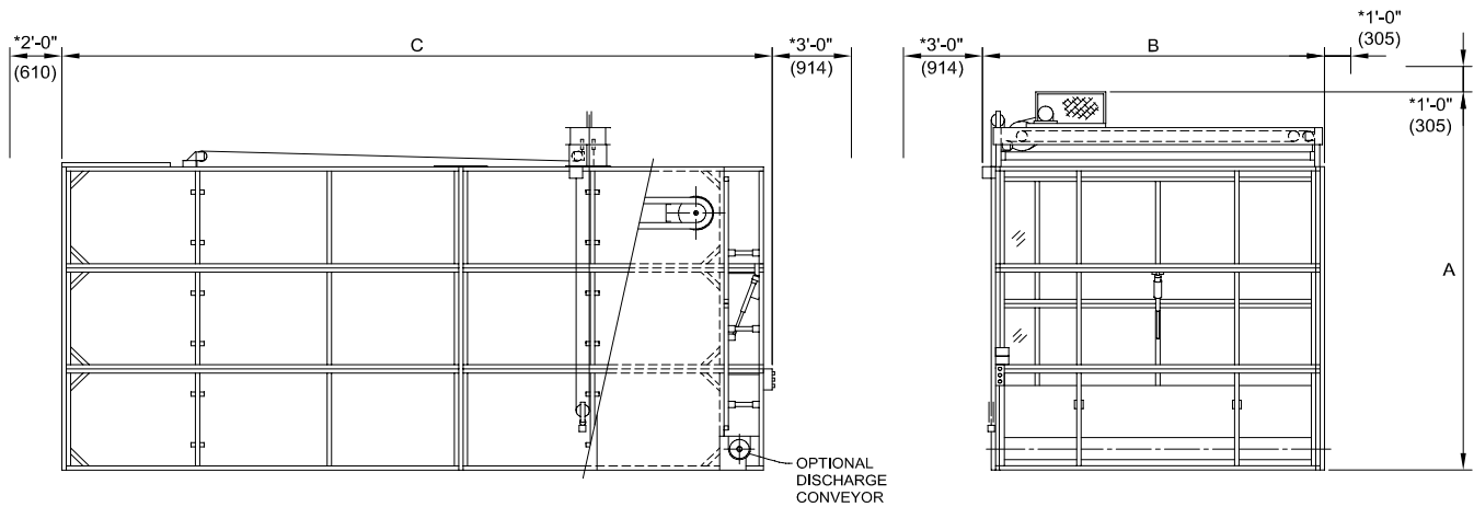
ELEVATION VIEW
